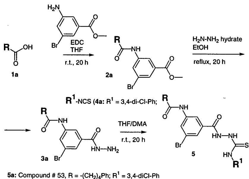
Scheme XIV
